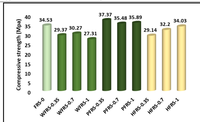
Figure 12 Compressive strength results
