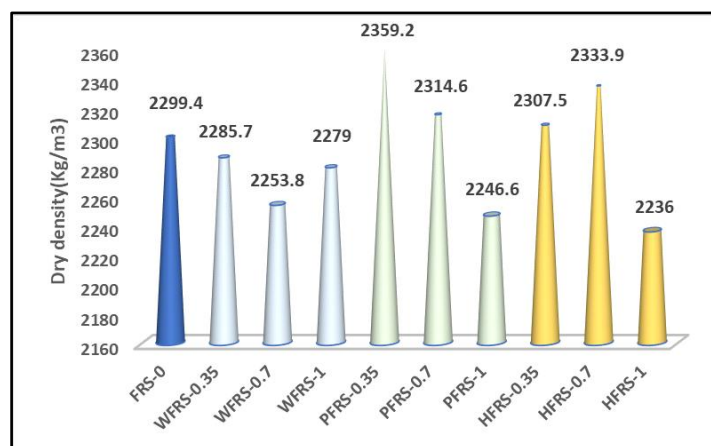
Fig. 9 Effect of fiber on the dry density of shotcrete
