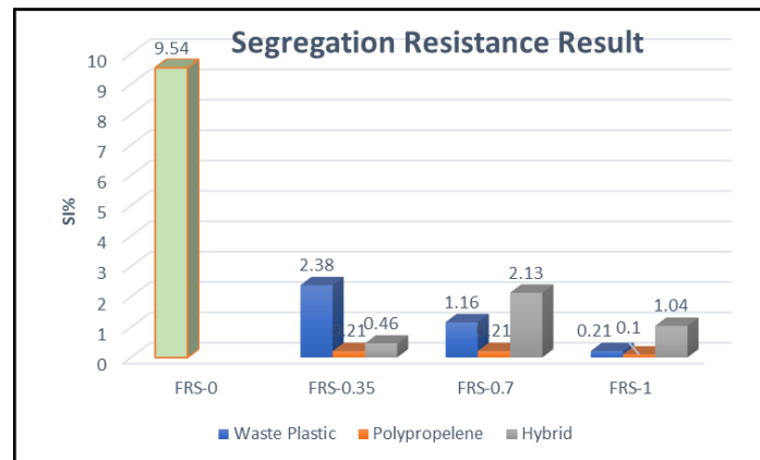
Fig. 6 Effect of fiber on the segregation resistance
