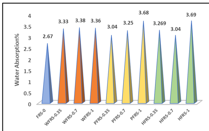
Fig. 8 Effect of fibers on the water Absorption
