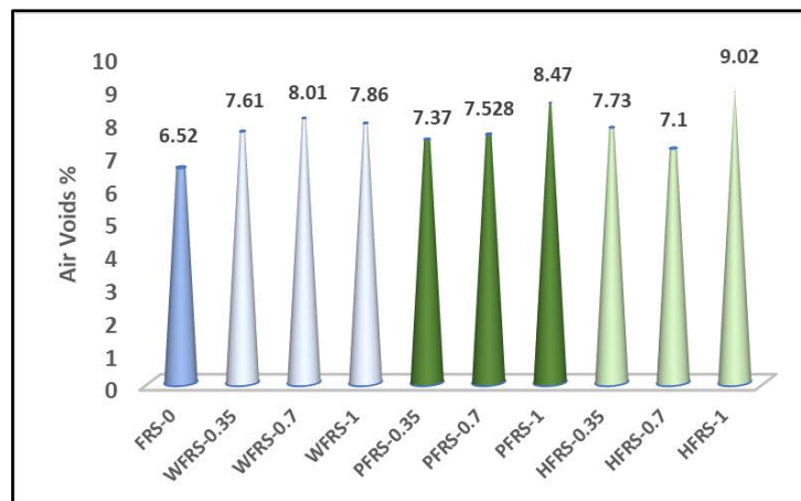
Fig. 7 Effect of fiber on the Air Voids.
