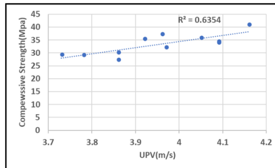
Figure 13 UPV and compressive strength relationship
