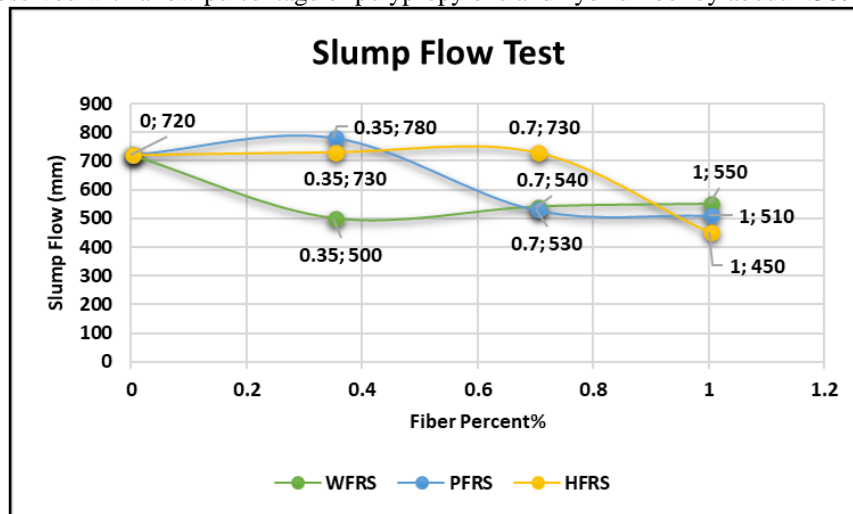
Fig. 4 Slump flow test results
