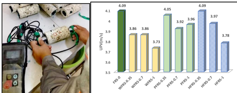
Fig. 10 Ultrasonic pulse velocity test and results
